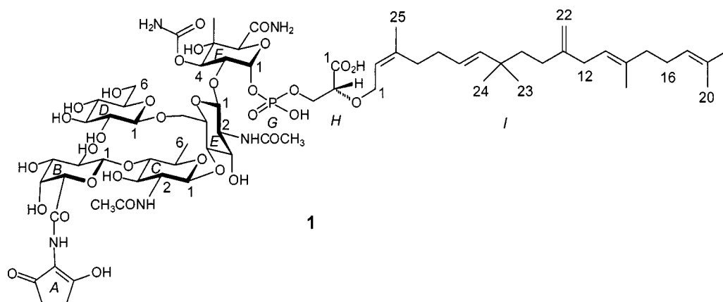
Figure 1. Moenomycin A
