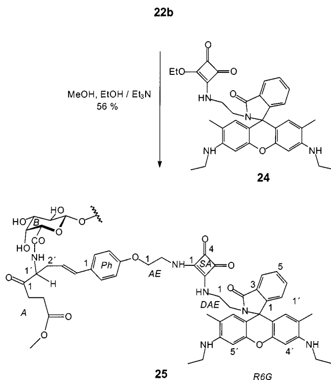
Scheme 9
